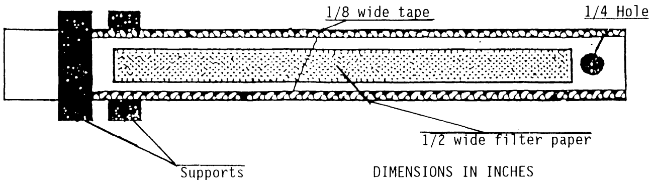
FIGURE 7. Crazing apparatus configuration.
